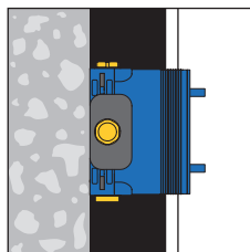
On-wall installation.
