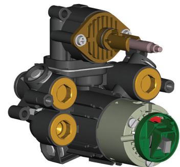
Single-lever mixer Choose between a bath and shower or shower fitting with CLICK-cartridge, hot water temperature control, ECO-function and DICHT-FIX.
