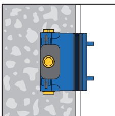
In-wall installation.
