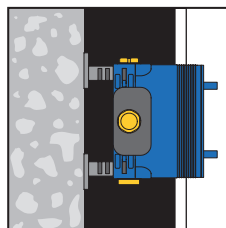
In-front-of-wall installation.
