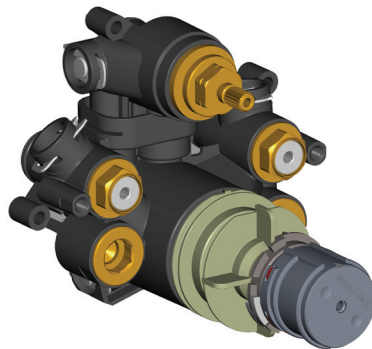
Thermostat Long-lasting thermostat cartridge, side valves for pre-shut off with non return valve and DICHT-FIX.
